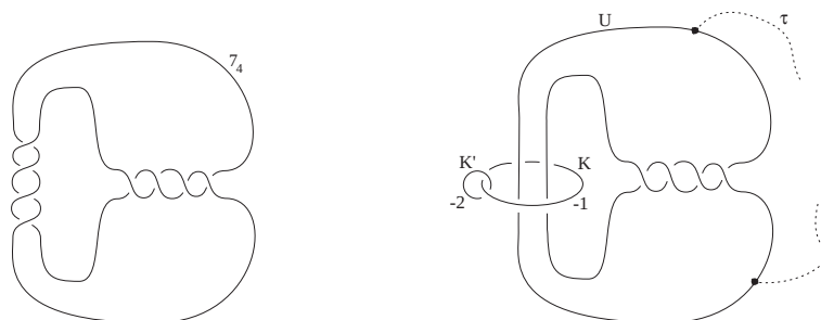
Figure 1: The knot 7_4
